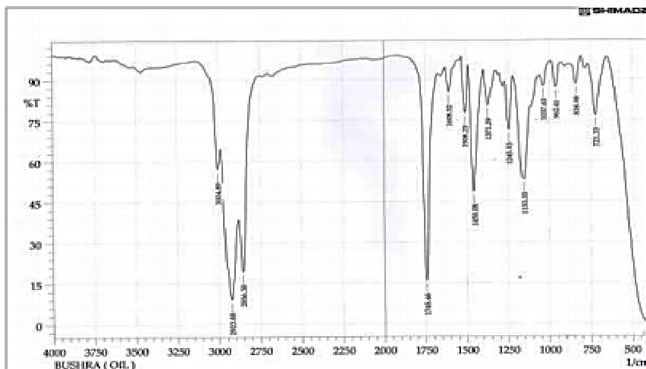
Figure(1): The full scan of IR spectrum for the oil extract of Anise ( pimpinella anisum L. ).
